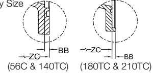
DETAIL C
