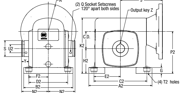
SSHF700 & SSHQC700 Hollow Shaft with Base
