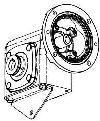
T Torque Arm (Shown assembled to SSH700 but ships separately as kit)
